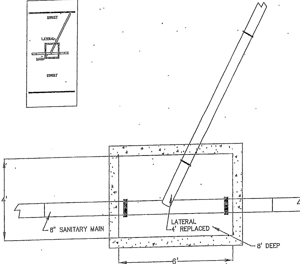
PLAN VIEW
