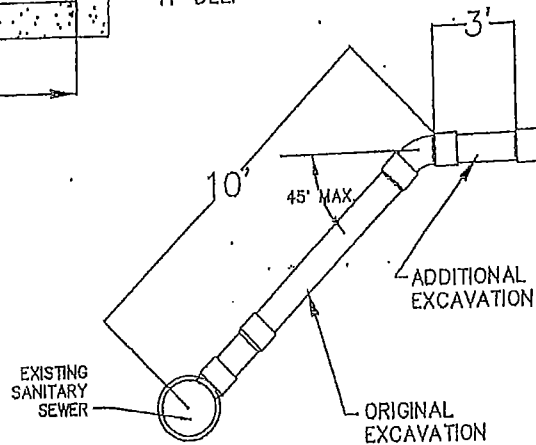
SECTION VIEW
