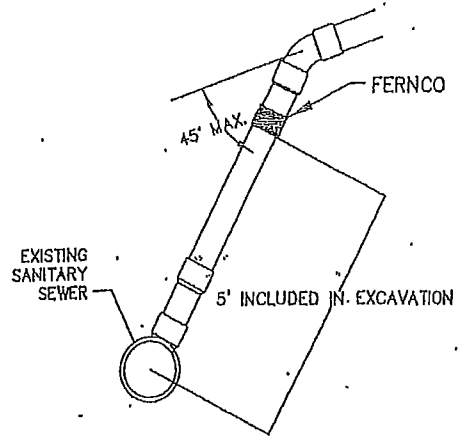
SECTION VIEW
